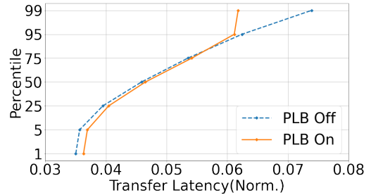
Figure 8: Latency for small ( \leq 1\text{KB} ) RPCs of storage workload
