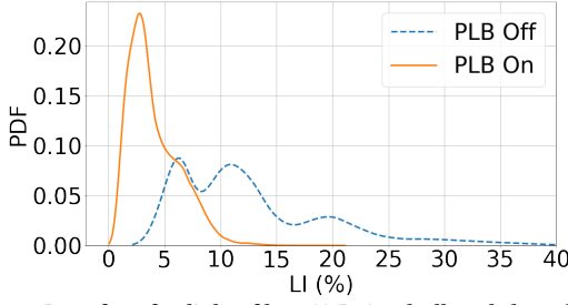
Figure 3: PDF of LI of uplinks of busy ToRs in a badly unbalanced data-center
