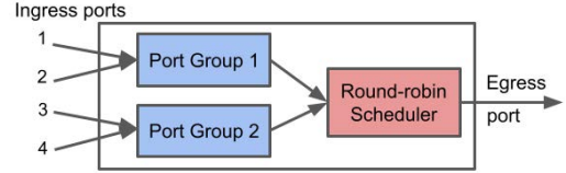
Figure 14: Scheduling over multiple port groups in a switch
