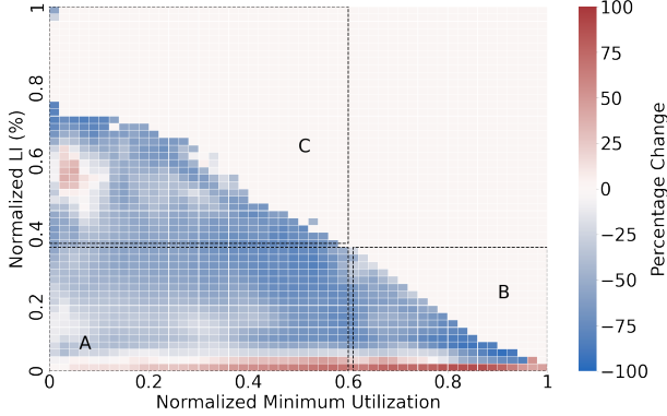
Figure 4: Percentage change in bin count after PLB is enabled where (x,y)=(\text{min\_utilization}, \text{LI}) . Red(hot) indicates increase in bin count whereas blue(cool) indicates a decrease.
