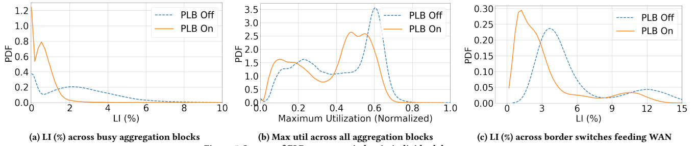
Figure 5: Impact of PLB on core switches in individual datacenters
