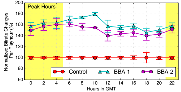
Figure 18: After switching to chunk map, the video switching rate of BBA-1 and BBA-2 is much higher than the Control algorithm.
