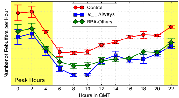
(a) Number of rebuffers per playhour.
