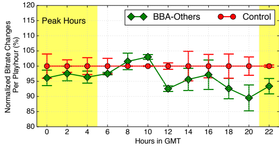
Figure 19: BBA-Others smoothes the frequency of changes to the video rate, making it similar to the Control algorithm.
