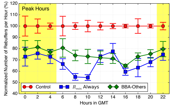
(b) Normalized number of rebuffers per playhour.
